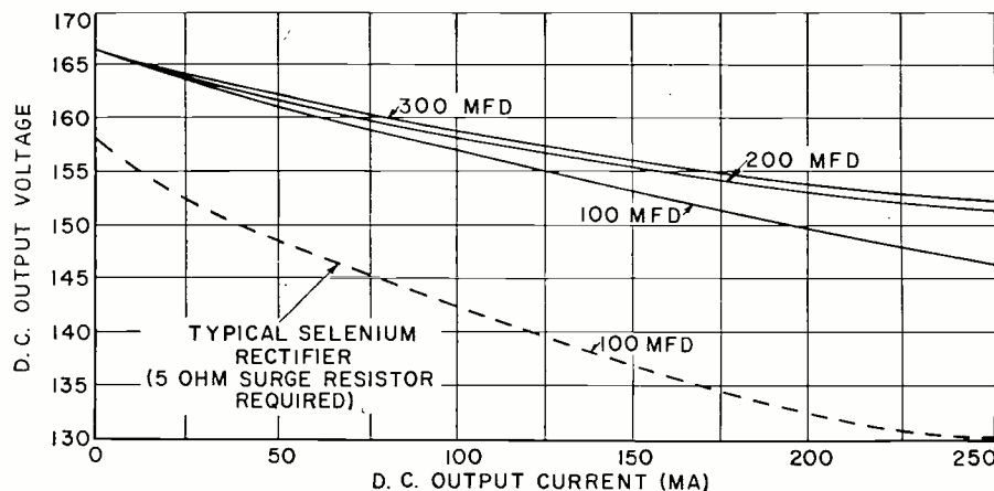
Fig. 2. Typical voltage regulation curves for the 1N573 germanium rectifier when used in a half-wave circuit with capacitive load, for three values of capacitance. A comparable curve for a selenium rectifier is also included.
