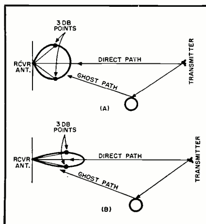
Fig. 4. A narrow-beamed, more directional antenna, like the one in (B), will reduce amplitude of the ghost.
