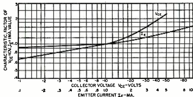
Fig. 6. Approximate curves showing variation of h_{fe} with collector voltage and emitter current for the General Electric low frequency "p-n-p" transistors.
