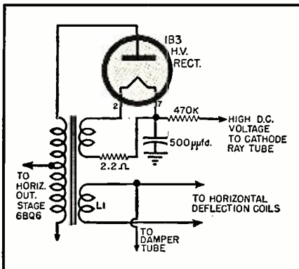
Fig. 1. A defective yoke winding unbalanced the h.v. transformer, reduced rectifier filament voltage, and killed h.v.
