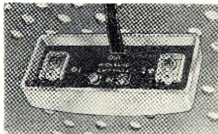
Fig. 2. Some interference can be tuned out with a receiver-installed high-"Q" frequency-selective adjustable trap.
