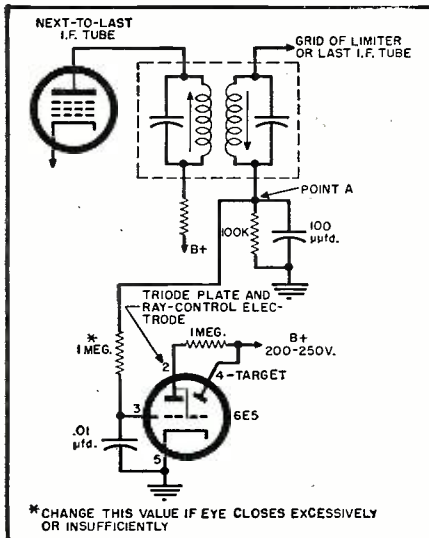
Fig. 2. Schematic diagram showing how 6E5 is connected for FM tuning indication.
