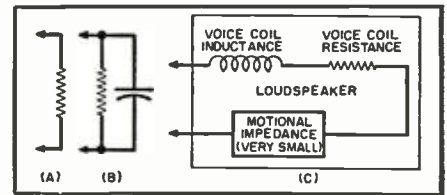
Fig. 2. (A) Common load used for testing although (B) is occasionally used. (C) Actual load offered by speaker to amplifier.
