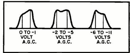
Fig. 5. Receiver i.f. circuits are designed for best response (center trace) over a certain normal range of a.g.c. voltage. Abnormally high signal level (right) can deteriorate performance as much as low signal and a.g.c. values.
