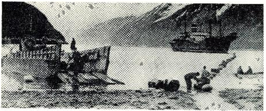
Beach landing of cable at Skagway, Alaska. The cable from the bow of the cable-ship Albert J. Myer, in background, is supported by means of drums and balloons.
