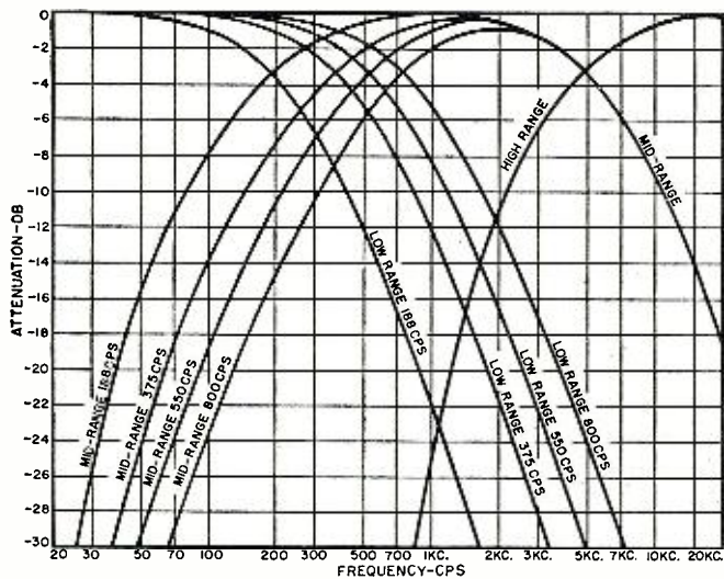
Fig. 6. Measured frequency response curves of three-channel amplifier.
