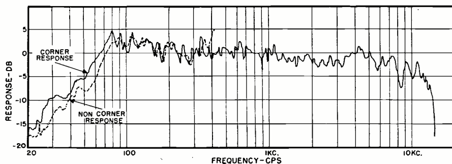
Relative response curves of the Model 6201 12-inch two-way speaker mounted in the "Tiny Mite" enclosure. Curves show comparative response with the enclosure placed in the corner of a room and against a flat wall. The corner position gives a somewhat better bass response, but only by about 3 or 4 db. Note also how the relative response falls off below approximately 80 cps at a rate of close to 12 db per octave.
