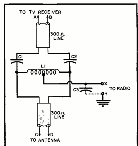
Filter gets double duty from TV antenna.
