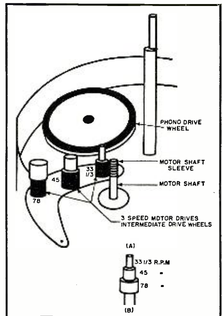
Fig. 1. Motion of motor, through its shaft, is transmitted to speed-changing drive wheel, to rubber drive wheel, to inner rim of turntable. Three separate intermediate drives for the various speeds are shown in (A). Sometimes a single shaft with three stepped diameters is used for speed changes, as in (B).
