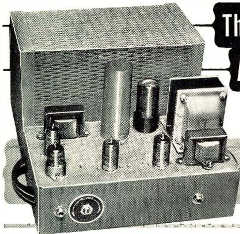
Fig. 1. Over-all view of consonant amplifier-limiter ("CA" limiter) is shown.
