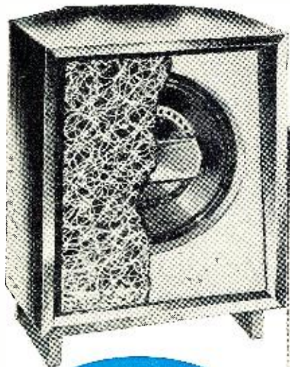
Cut-away assembly views of the "Tiny Mite" showing installation of an integrated 12" 3-way speaker and a 3-way system using an 8" 2-way speaker and a separate tweeter.
