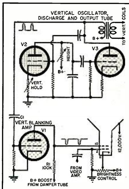
Fig. 2. A vertical circuit fault dimmed the raster. Excessive conduction of the blanking amplifier reduced voltage on the accelerating anode of the picture tube.
