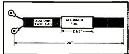
Fig. 6. Tuned line is used to locate interference frequency or act as trap.
