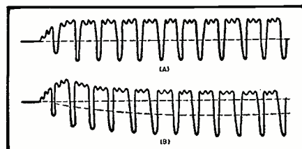
Fig. 4. (A) Asymmetric wave without isolating d.c. (B) Offsetting bias adjustment.
