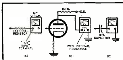
Fig. 2. Resistor added (A) to increase impedance. When meter's internal resistance (B) puts d.c. load on circuit under test, use an isolating capacitor (C).
