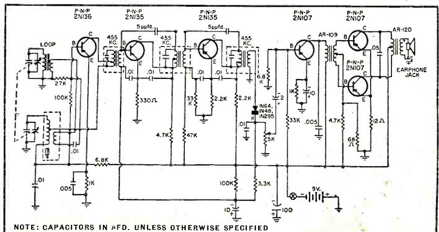
Schematic diagram of six-transistor superhet. Special parts are used extensively.
