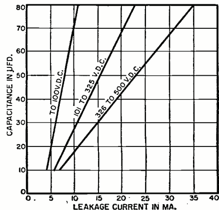
Fig. 2. Leakage for a given combination of capacitance and voltage rating should not exceed values shown here.
