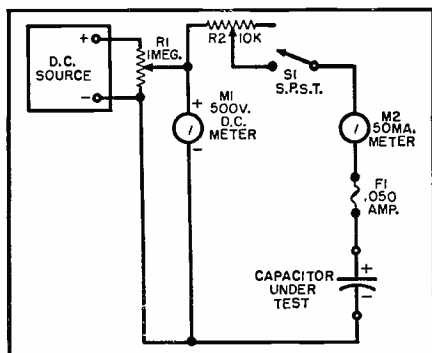
Fig. 1. Leakage current through capacitor is measured at rated voltage with the simple test circuit depicted here.
