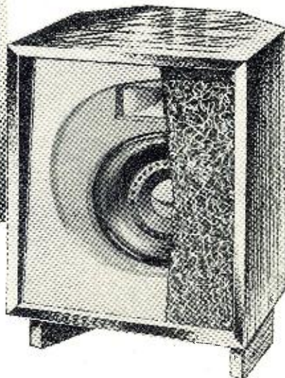
Cut-away assembly views of the "Tiny Mite" showing installation of an integrated 12" 3-way speaker and a 3-way system using an 8" 2-way speaker and a separate tweeter.
