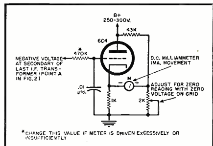
Fig. 8. Simple schematic diagram showing use of conventional d.c. milliammeter connected to driver tube for signal strength indication.
