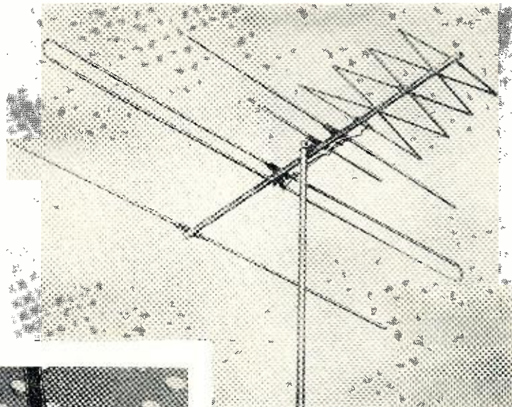
Fig. 1. The JFD "Super Helix" is an example of an antenna with a narrow polar angle (see Fig. 4B) that weakens ghosts.
