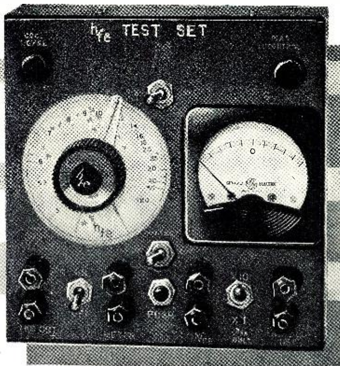
Fig. 1. Front panel view of transistor test set that measures current gain.
