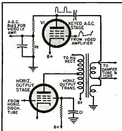
Fig. 3. Trouble in the horizontal amplifier reduced the flyback pulse. Although the raster appeared unaffected, operation of the keyed a.g.c. stage was disturbed.
