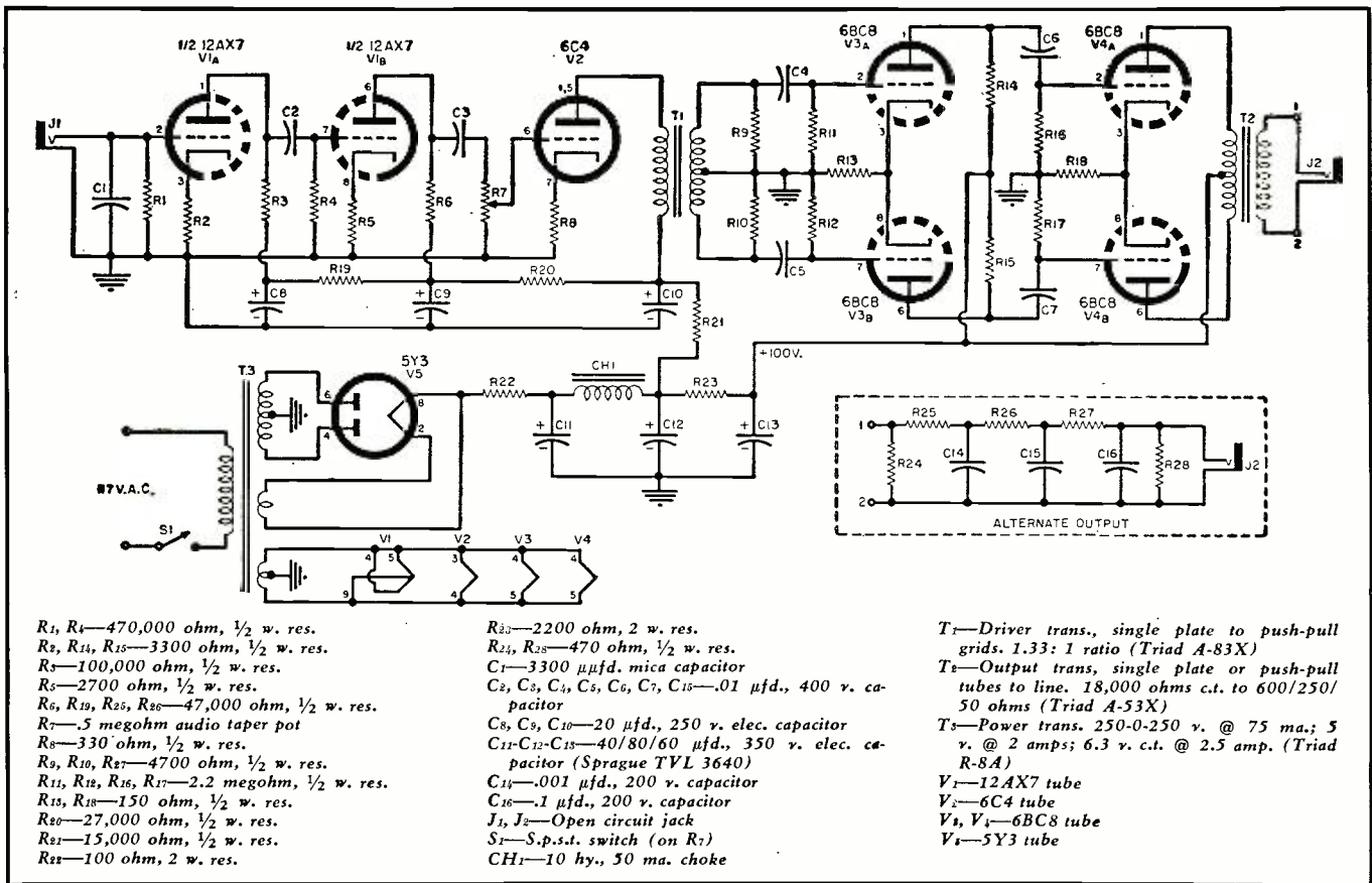
Fig. 4. Complete schematic diagram of the consonant amplifier-limiter circuit. A 12AX7 is utilized as a two-stage pre-amplifier for the 6C4 driver stage. This, in turn, feeds the pair of 6BC8's operating as a two-stage push-pull grid bias limiter.
