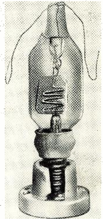
Early deForest audion. This picture came from the late Sir Ambrose Fleming together with a label in his handwriting worded "deForest original valve or Audion. 1907." The over-all height of the tube, including the screw base, is about 3¾ inches.
