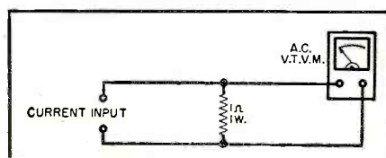
Fig. 5. External shunt resistor (1-ohm non-inductive) converts the v.t.v.m. into an a.c. ammeter or milliammeter.
