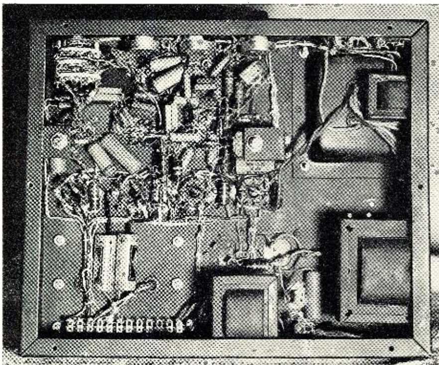
Fig. 7. Under-chassis view of the completed three-channel audio power amplifier.
