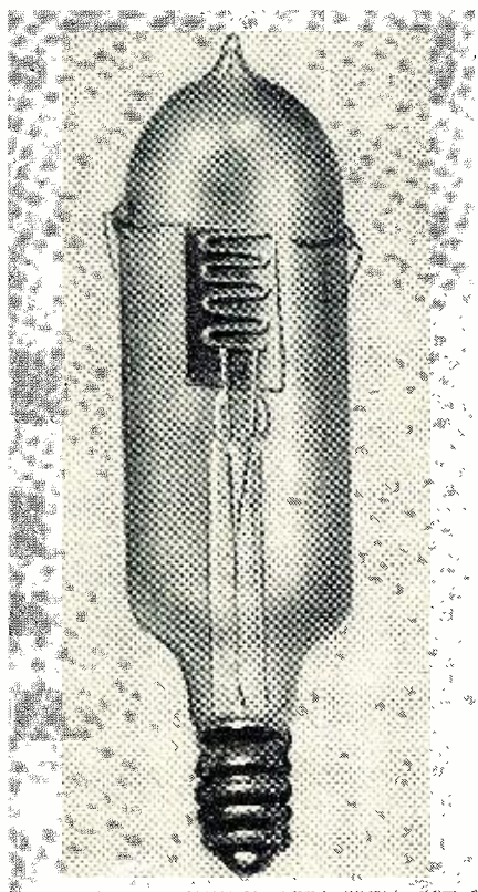
Photograph of the earliest type of three electrode audion tube, with the grid and plate leads brought out through the side walls of the cylindrical glass envelope. Filament leads are connected to screw base.
