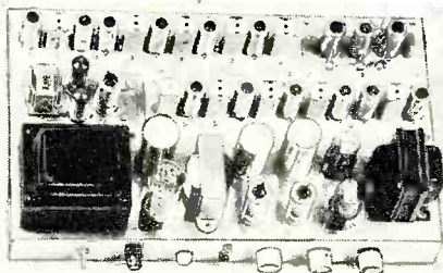
Fig. 2. Top-chassis view of a multiplex receiver made by Collins Audio Products.
