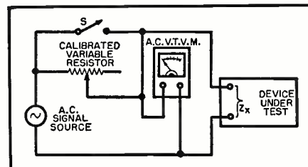
Fig. 3. Checking an unknown impedance.
