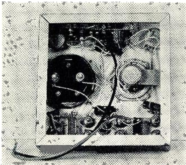
Fig. 5. Under-chassis view of the transistor test set. The 2N107 transistor used as the phase-shift oscillator is mounted on the fiber board at the top of the photo.
